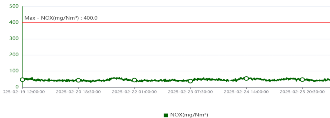
Fig. – 2 & 3: OCEMS of HURL Sindri, Ammonia Stack Reformer
