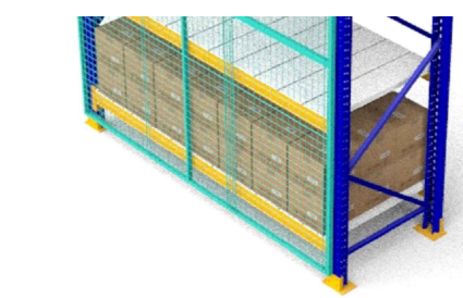
Mesh Cladding(Tube) Grid Size (50x50) Extremes sides of racks (Shown in "#")
