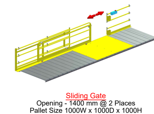
Sliding Gate Opening - 1400 mm @ 2 Places Pallet Size 1000W x 1000D x 1000H
