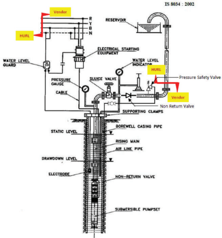
FIG. 2 TYPICAL SUBMERSIBLE PUMPSET INSTALLATION
